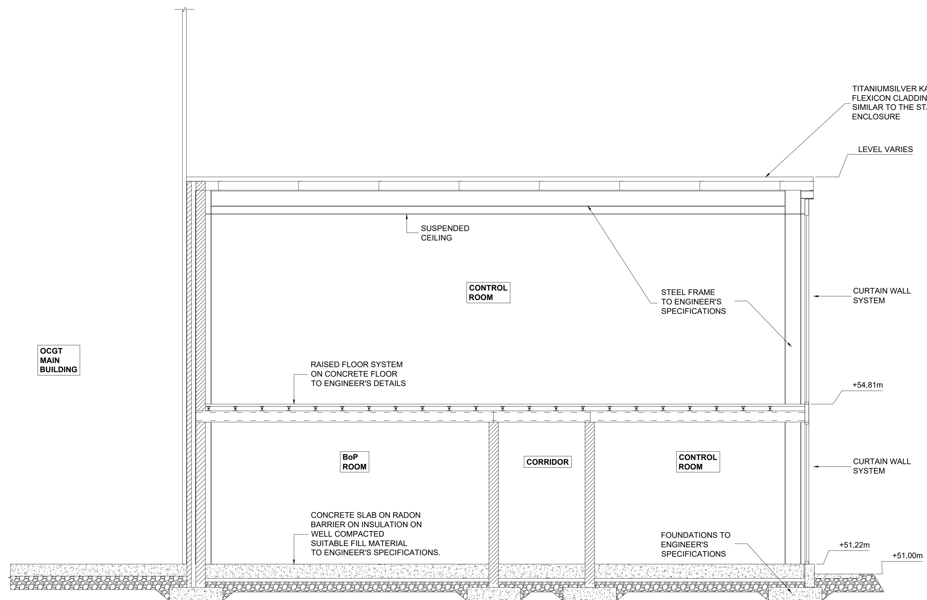
SECTION 2-2 SCALE 1:50
