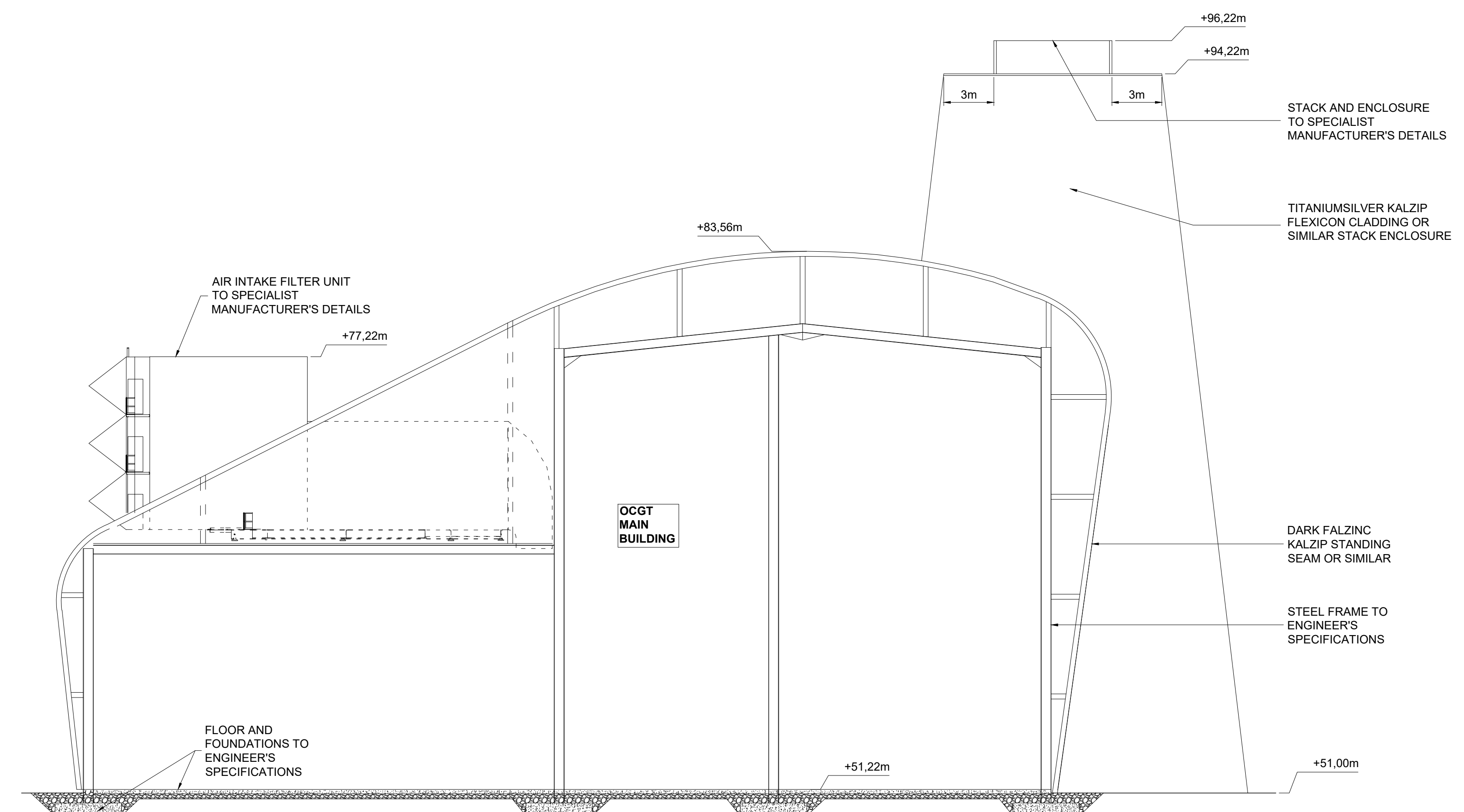
SECTION 1-1 SCALE 1:200
